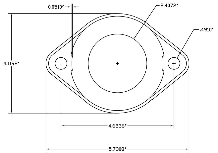
2" DISCHARGE FLANGE
